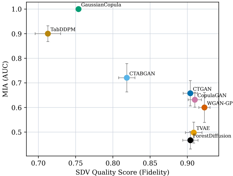
Air Quality: SDV Quality Score (Fidelity) vs MIA (AUC)
